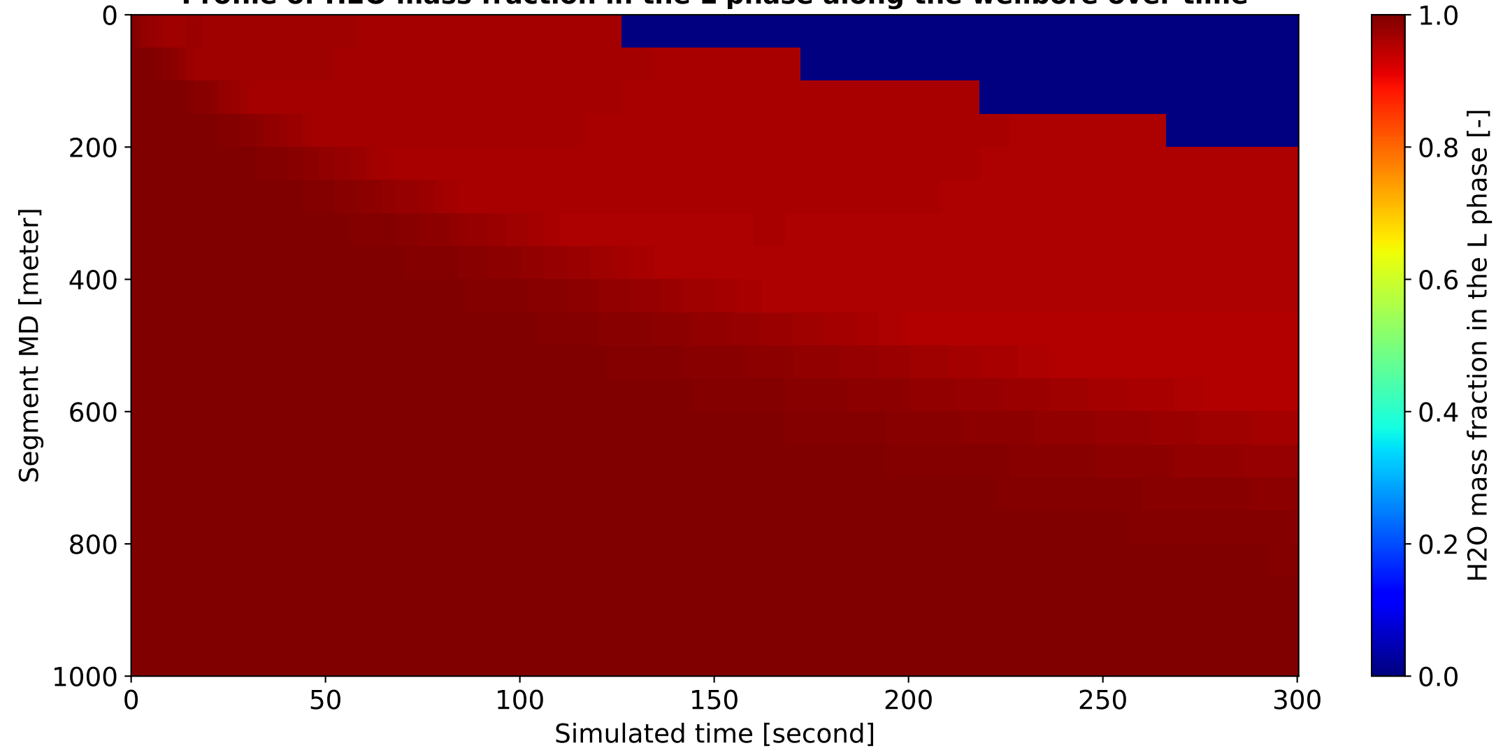
Profile of H2O mass fraction in the L phase along the wellbore over time
